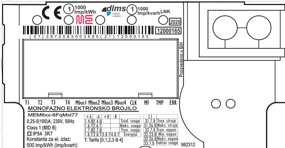
Figure 2: Front plate of MEM6xx electricity meter
