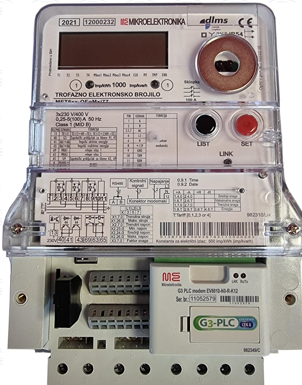
Figure 2: View of MET6xx-OFpqwC77 Three-phase electronic electricity meter without terminal cover
