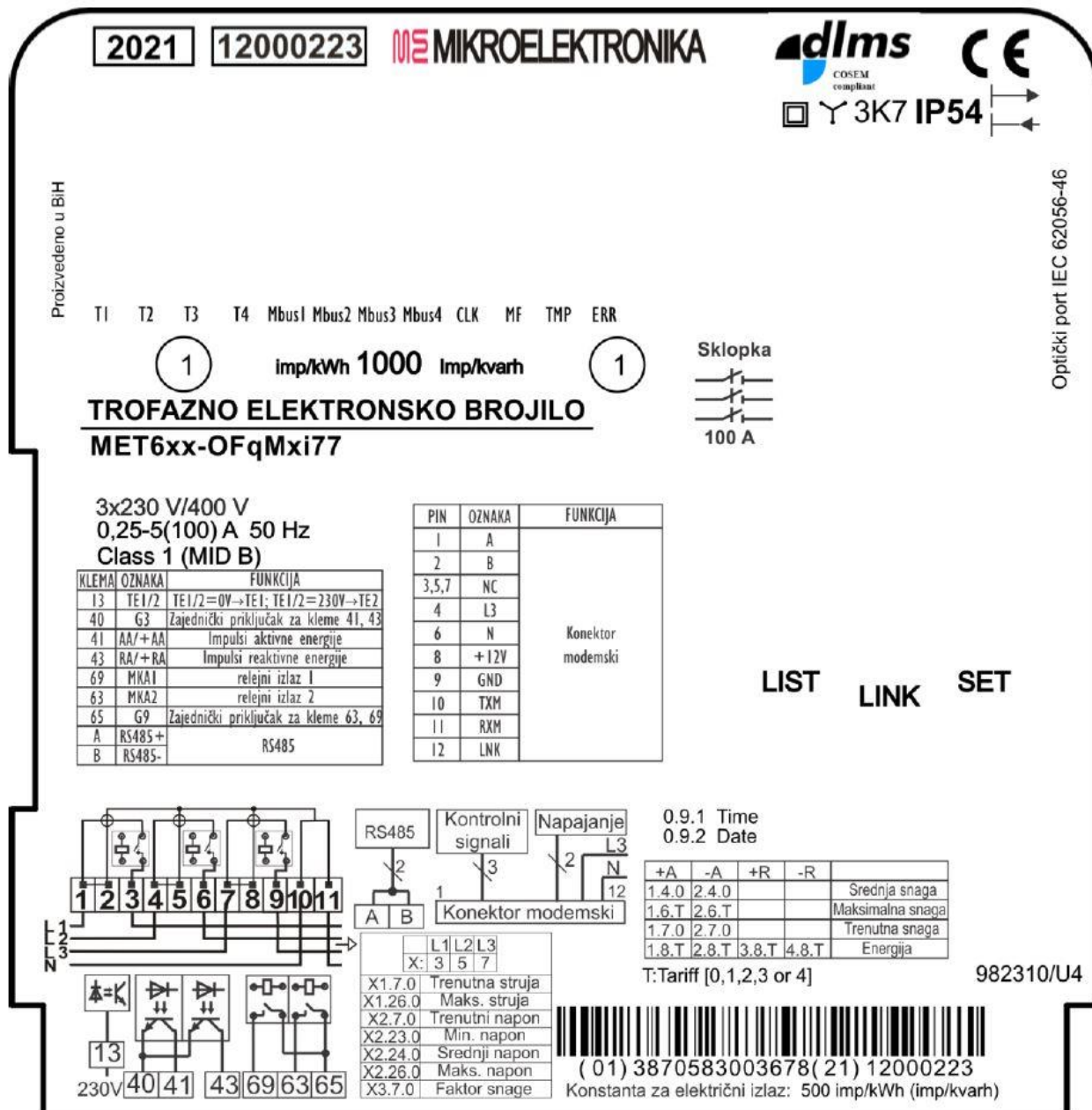
Figure 3: Front plate of MET6xx-OFpqrC77 electricity meter
