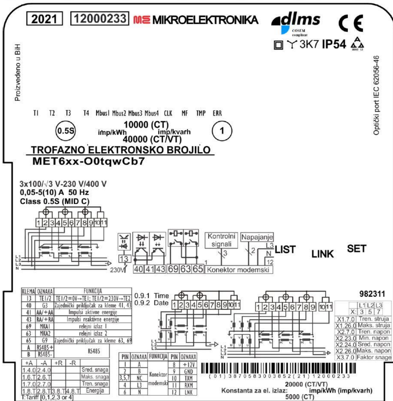
Figure 3: Front plate of MET6xx-O0tqwCb7 electricity meter
