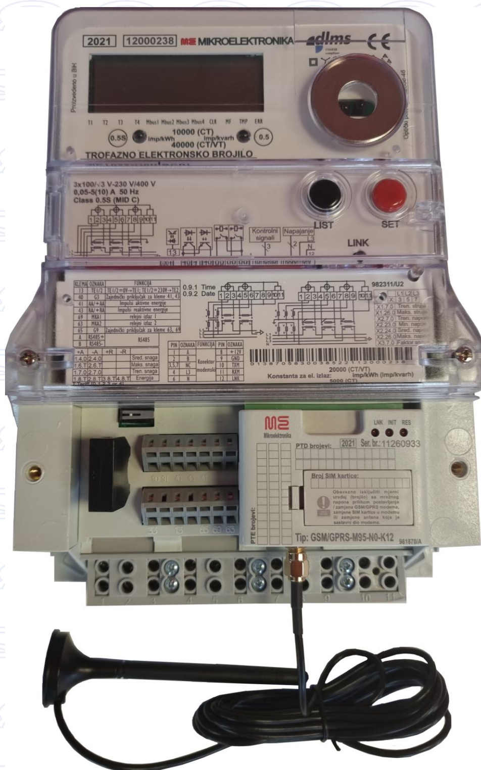
Figure 2: View of MET6xx-O0tqwCb7 Three-phase electronic electricity meter without terminal cover
